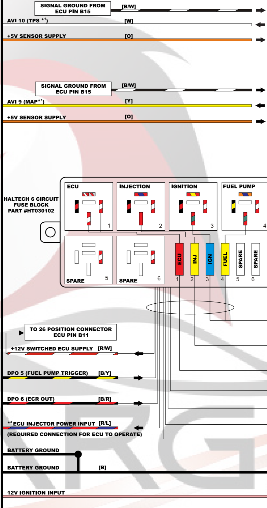
MANIFOLD ABSOLUTE PRESSURE SENSOR
